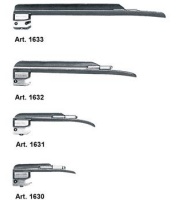
1640 Miller Laryngoscope set with 4 standard light blades
